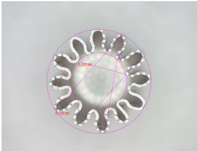
Outer Circle Diameter of a Pleated Filter: 3.10mm Outer Circle Diameter of a Pleated Filter: 1.68mm
