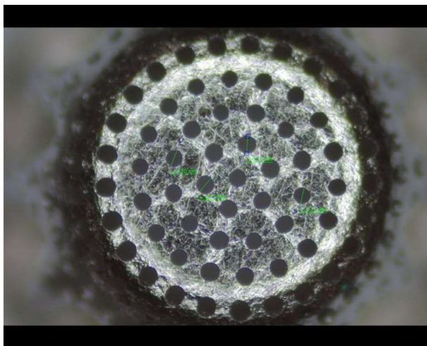
Pleater Filter Micro Hole Diameter : \Phi 0.10-0.11mm
