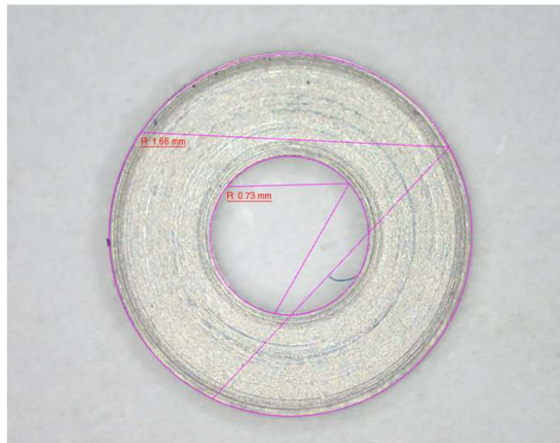
Flange Outer Diameter: \Phi 3.32 Flange Inner Diameter: \Phi 1.46
